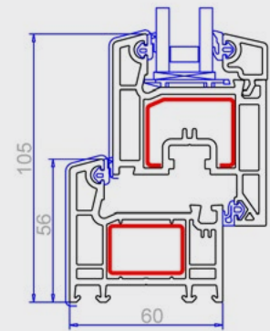
↑ Window Acryl-Color COEX
