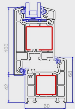
↑ Window Acryl-Color COEX
